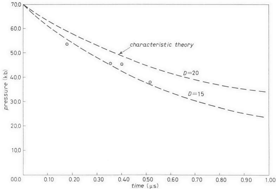
Fig. 20. - Precursor decay in single crystal tungsten, courtesy of T. E. MICHAELS, W.S.U. (unpublished).
